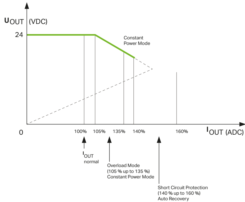
Figure 8: Overload Behavior
