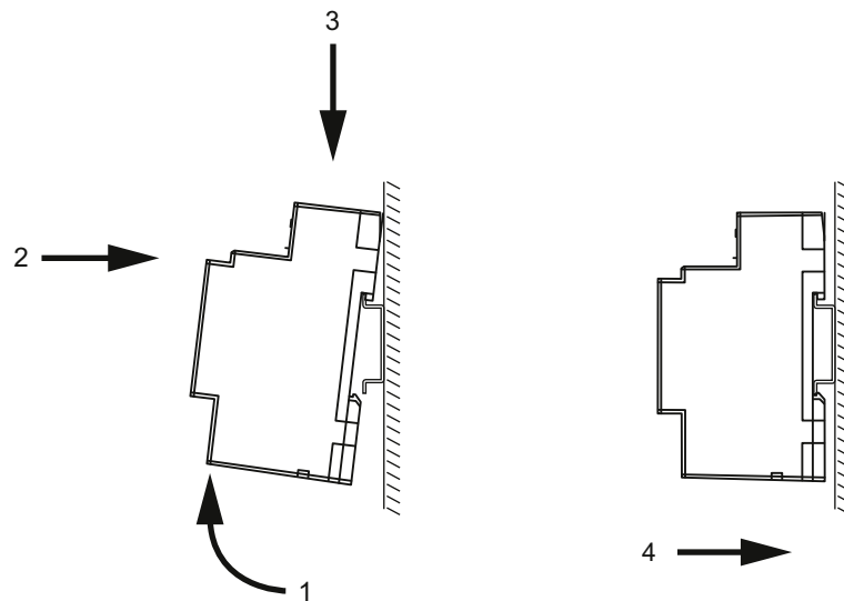
Figure 15: Mounting the Product on the DIN rail
