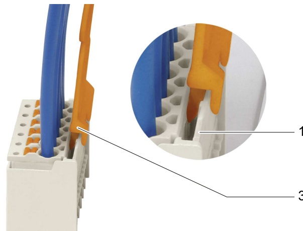
Figure 20: Removing the Female Connector with Wiring (Application Example)
