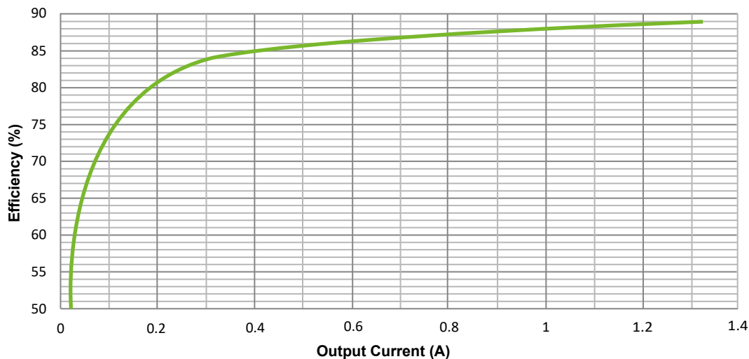
Figure 11: Efficiency at 230 VAC
