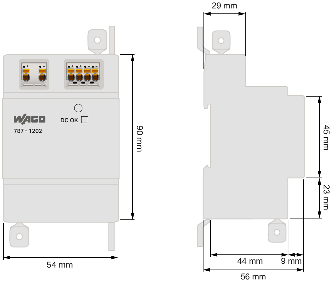
Figure 7: Dimensions
