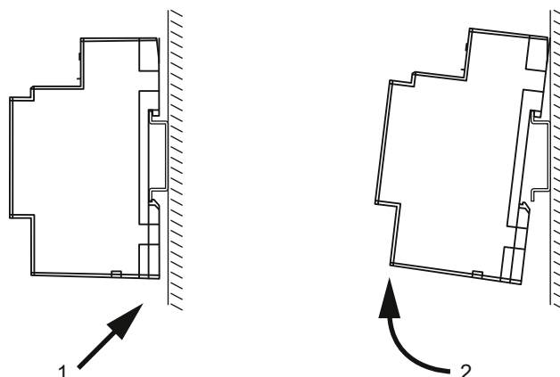
Figure 16: Removing the Product from the DIN Rail
