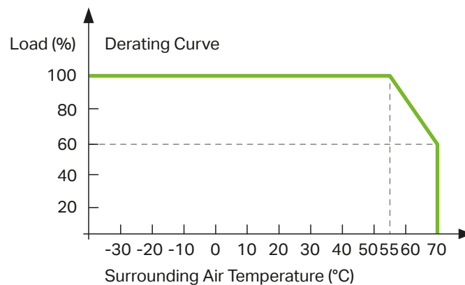
Figure 13: Derating surrounding air temperature
