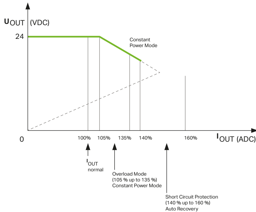
Figure 22: Output Characteristics
