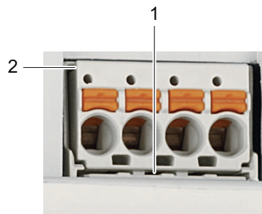
Figure 19: Removing the Female Connector without Wiring (Application Example)
